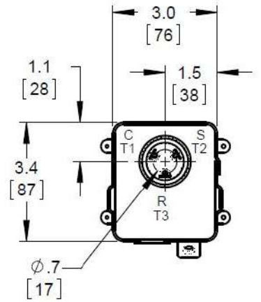
TERMINAL BOX (QUICK CONNECT TERMINALS)
